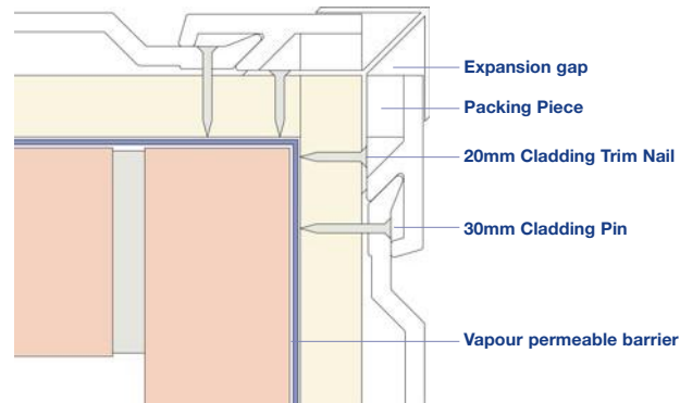
External Corner - Vertical Installation
