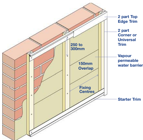
Batten Installation - Kavex Only
